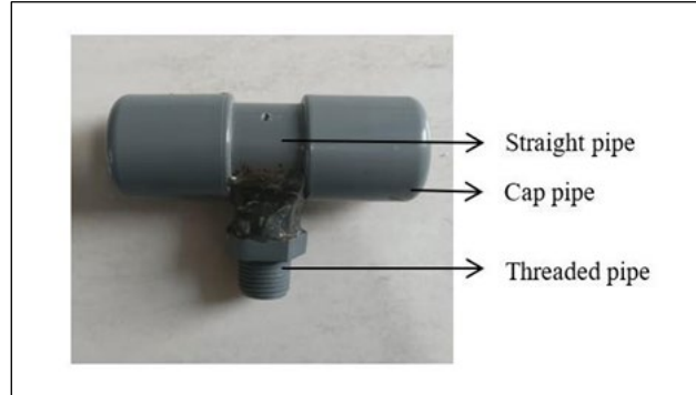
Figure 1. Ventury dual nozzle
